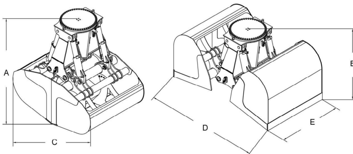
Fig. 2: Dimensioned drawing of the grab
